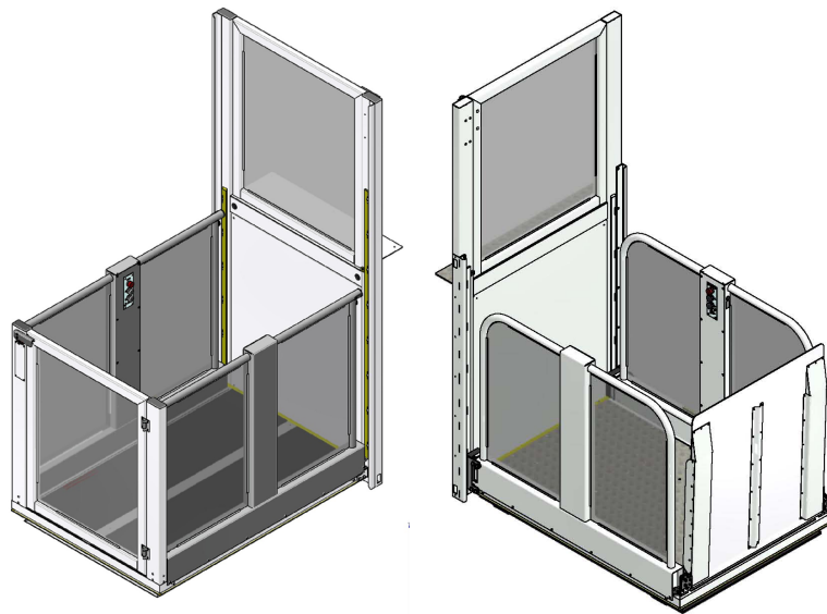
Schematic views of units with a door on the platform and with a access ramp on the platform
